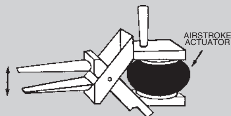
CORE STRAIGHTENER
