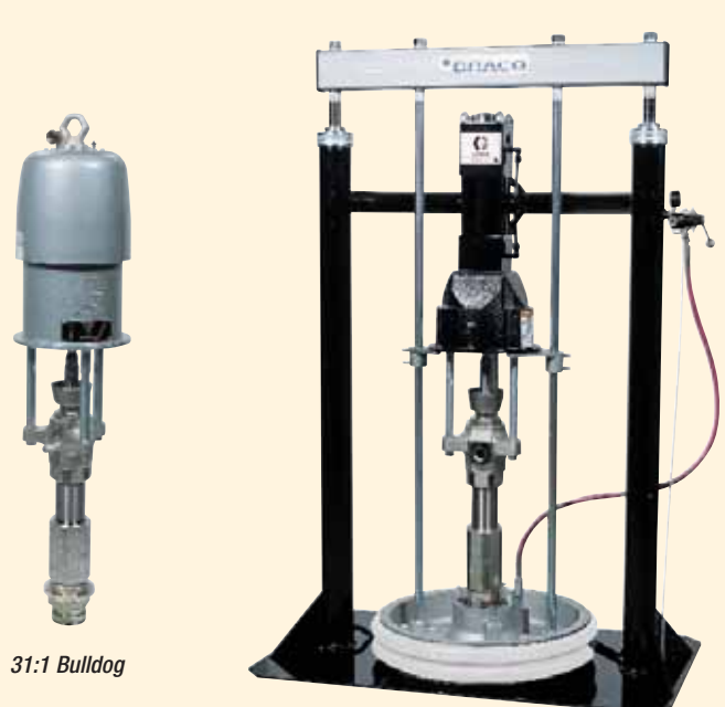
Viscount II 3100 on 55 gallon ram
