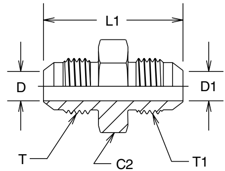
C2*—LARGE HEX ALLOWS FOR USE IN MS33649 PORT
