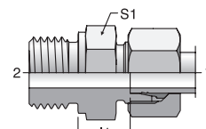
Cutting face DIN 3852, form B, G (BSPP) thread
