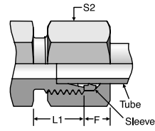
EO/EO-2 Assembly
