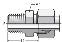
R (BSPT) thread
