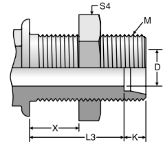
EO/EO-2 Bulkhead
